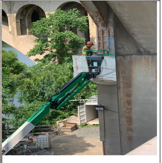
Concrete repair at East ramp by the use of manlift
