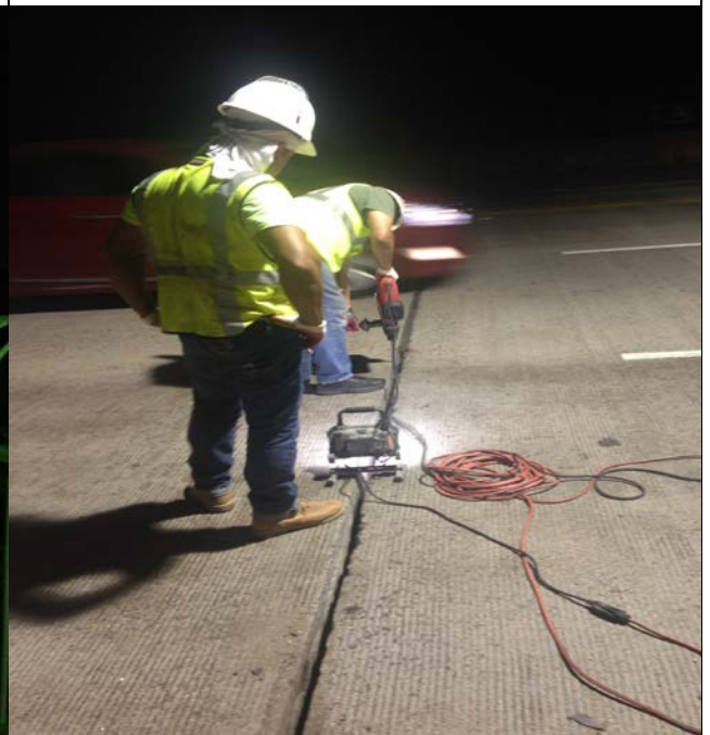
Drilling Core Sample for shotcrete compressive strength
